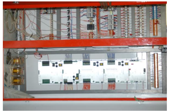
AIR CONDITIONING CONTROLS
